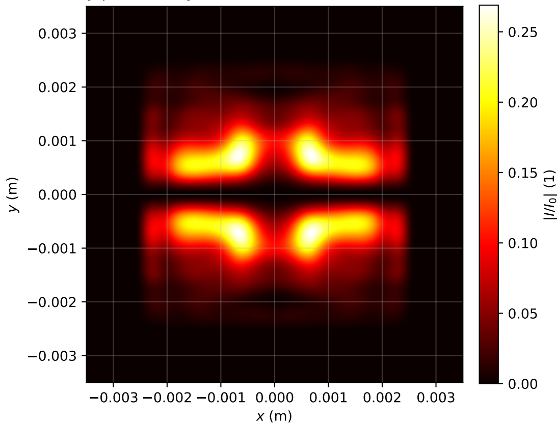
Intensity profile I(x, y, z = 3.821)/I_0 , \text{Pin}=4.0\text{Pcr} , artificial time
